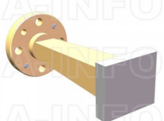
LB-15-10-ASPO Standard Gain Horn Antenna 50-75GHz 10dB Gain Rectangular Waveguide Interface
